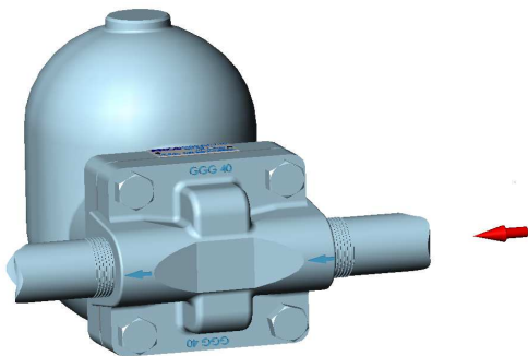
Correct Installation
