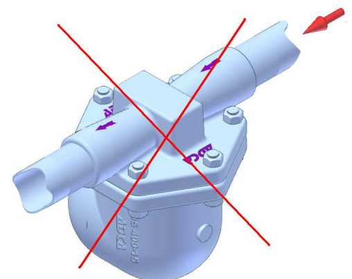
Wrong Installation
