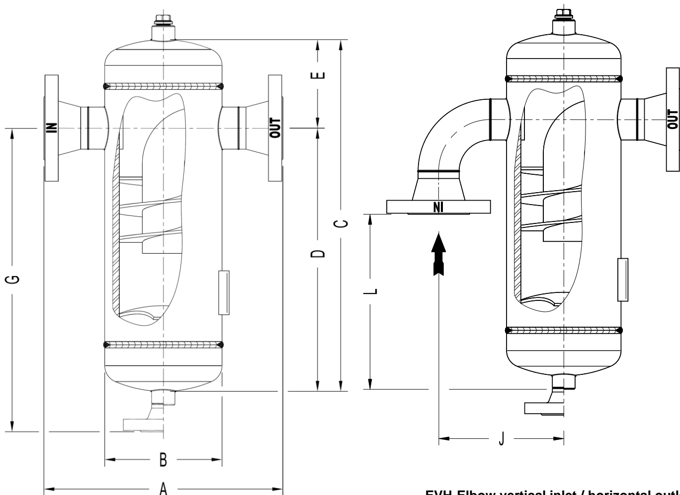
EVH-Elbow vertical inlet / horizontal outlet
